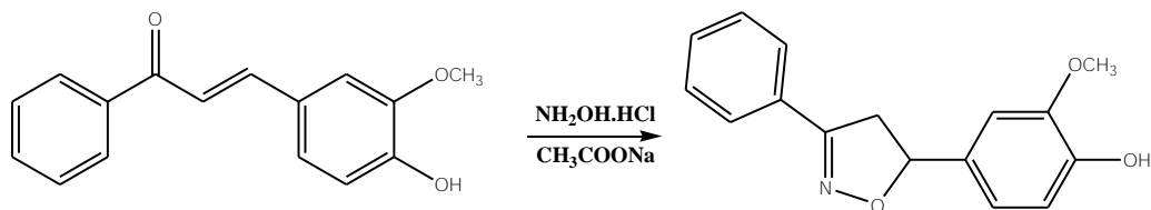
Gambar 6. Reaksi Sintesis Isoksazola
